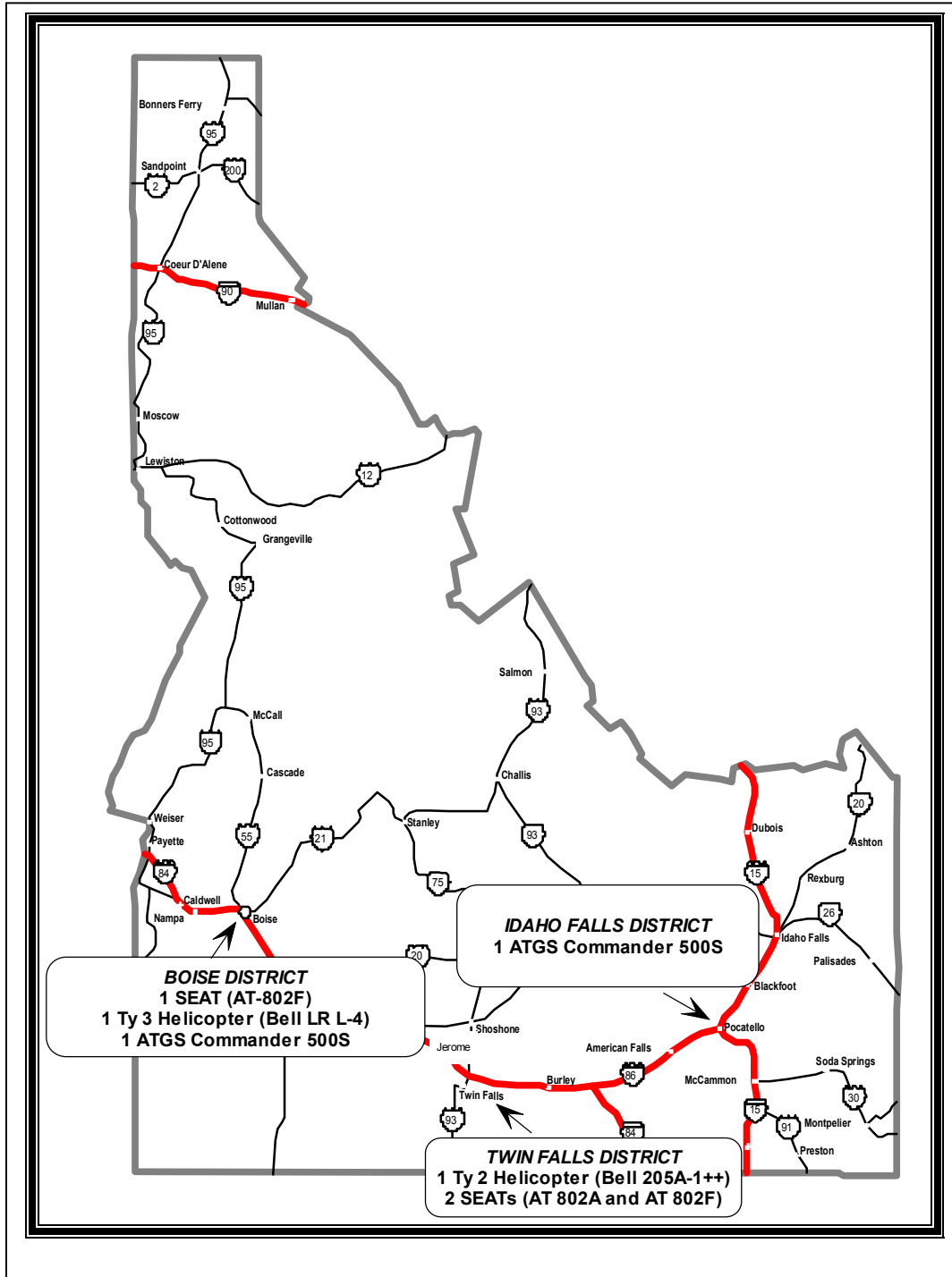
Figure B-1: Location of Idaho BLM Exclusive-Use Contract Aircraft
